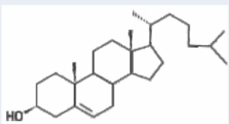
Cholesterol
